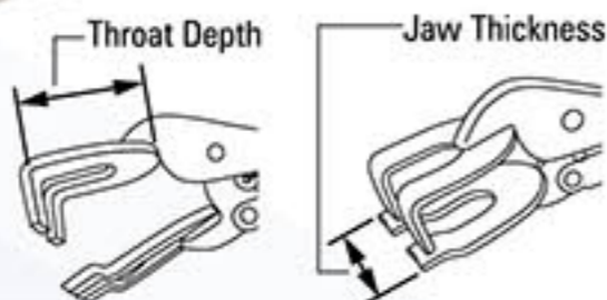
Throat Depth: 2-3/16" (55.5 mm) Jaw Thickness: 0~2-3/4" (0~69.8 mm)
